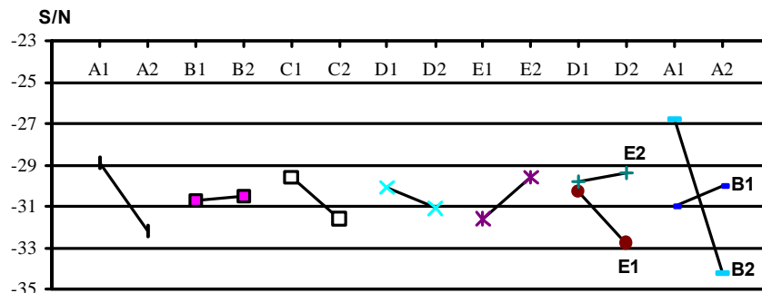
Figure 1 Response graphs for major effects and major interactions
