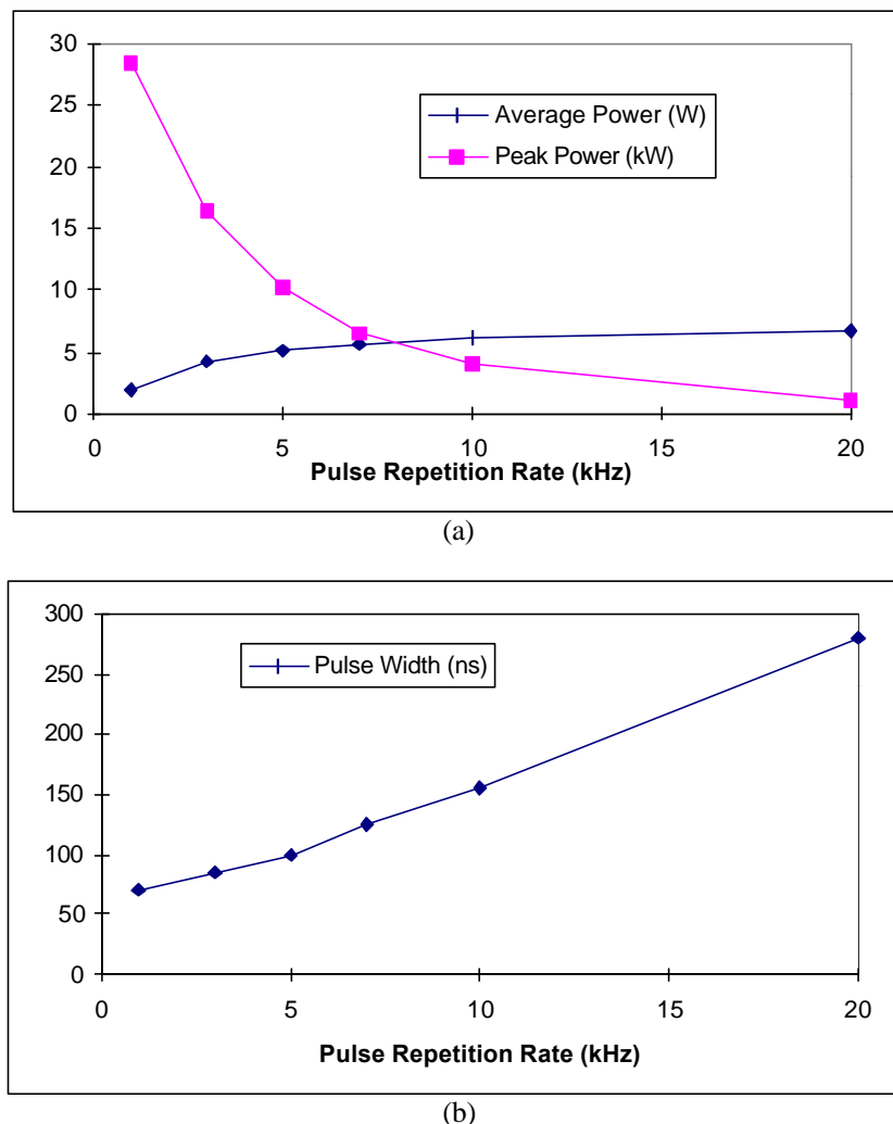
Figure 3 Laser performance at different pulse repetition rate: (a) peak power and average power; (b) pulse width
